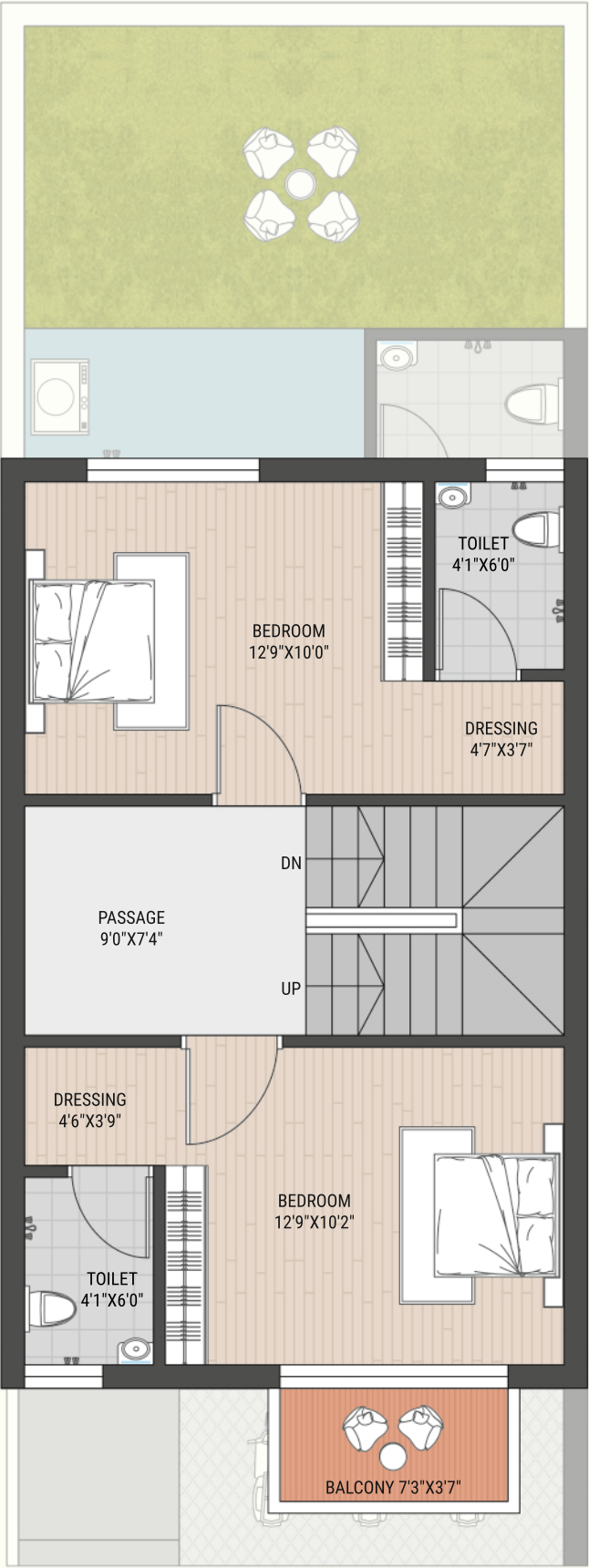
FIRST FLOOR - 2 BEDROOM
