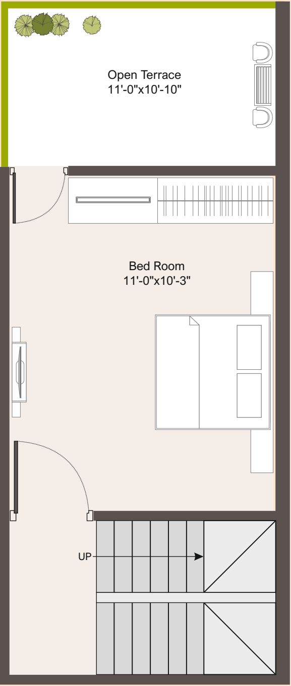
SECOND FLOOR PLAN Total Sq. Ft. 183.77
